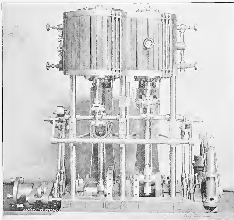
COMPOUND YACHT ENGINE, WITH AIR AND FEED-PUMP ATTACHED.—Designed and Built by the Edward S. Clark Co., Boston, Mass.
